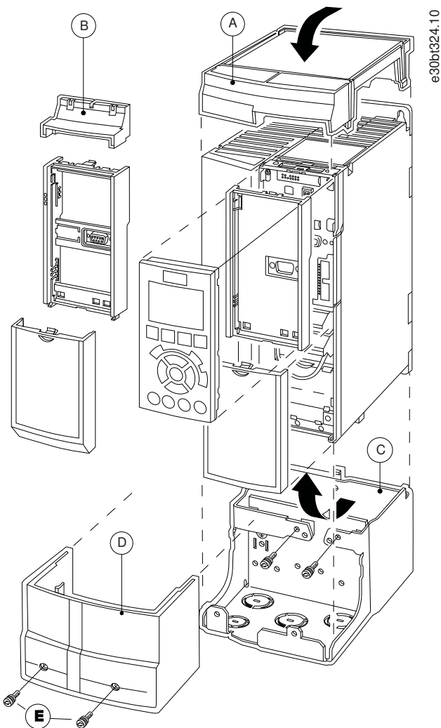
Illustration 44: IP21/Nema Type 1 Kit on A3 Enclosure
