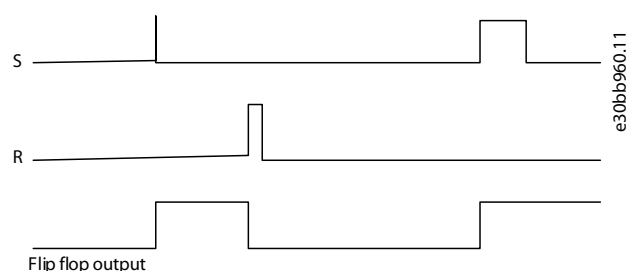
Illustration 40: Flip Flop Outputs
