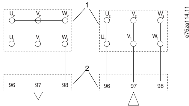
Illustration 62: Motor Cable Connection
