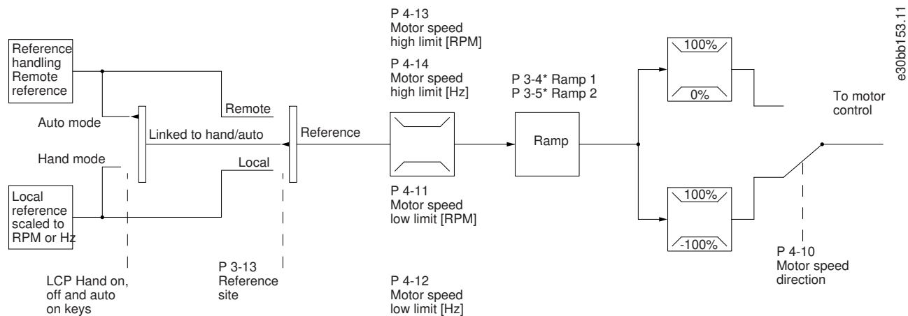
Illustration 91: Open-loop Structure
