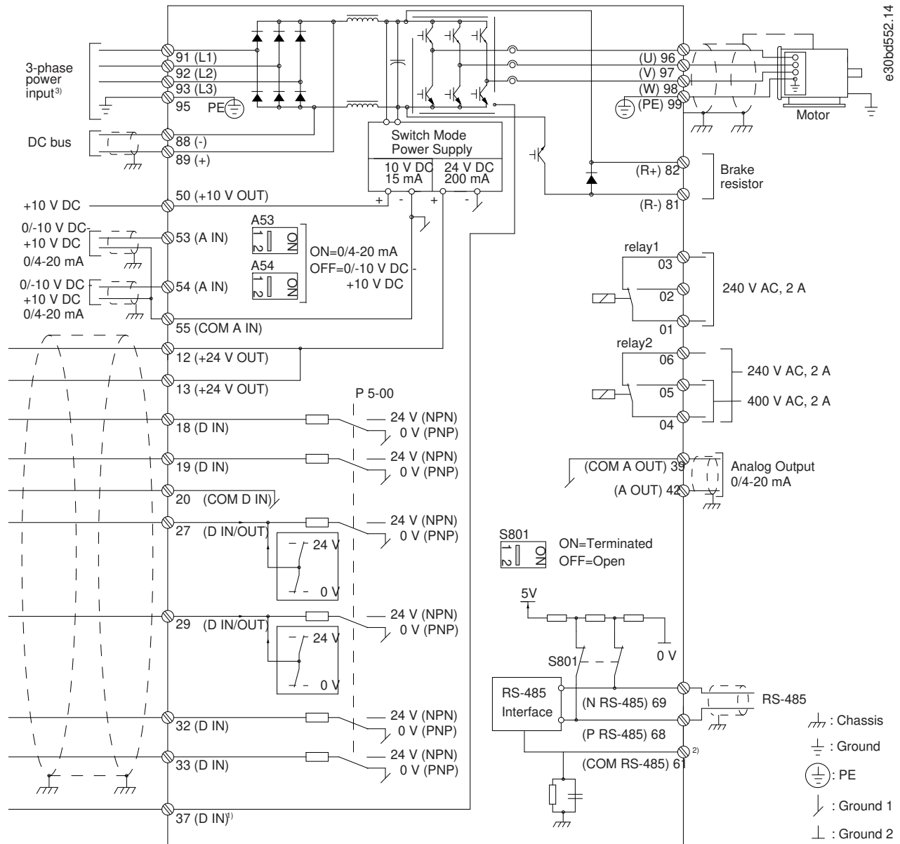
Illustration 59: Basic Wiring Schematic
