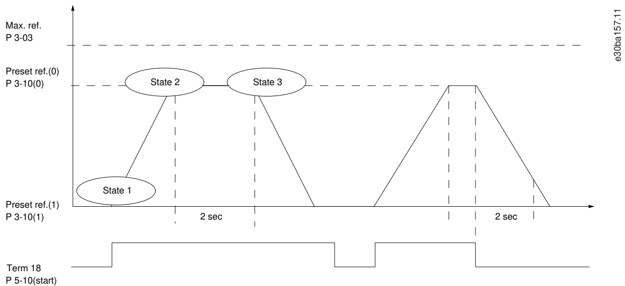
Illustration 37: Application Example, Ramp Up/Ramp Down
