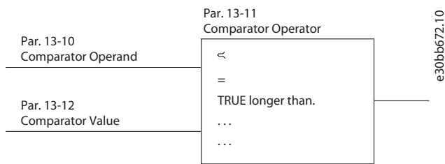
Illustration 35: Comparators
