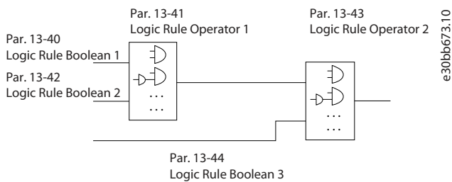
Illustration 36: Logic Rules
