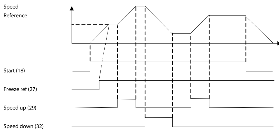
Illustration 93: Speed Up/Down
