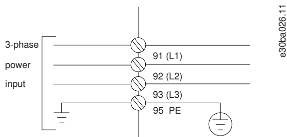
Illustration 61: Connection of Mains
