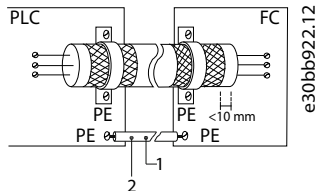
Illustration 64: Shielding Clamps at Both Ends
