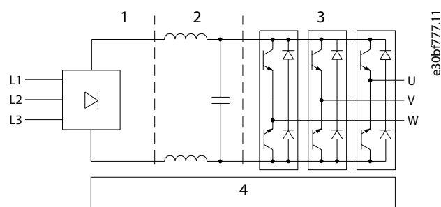
Illustration 84: Internal Processing
