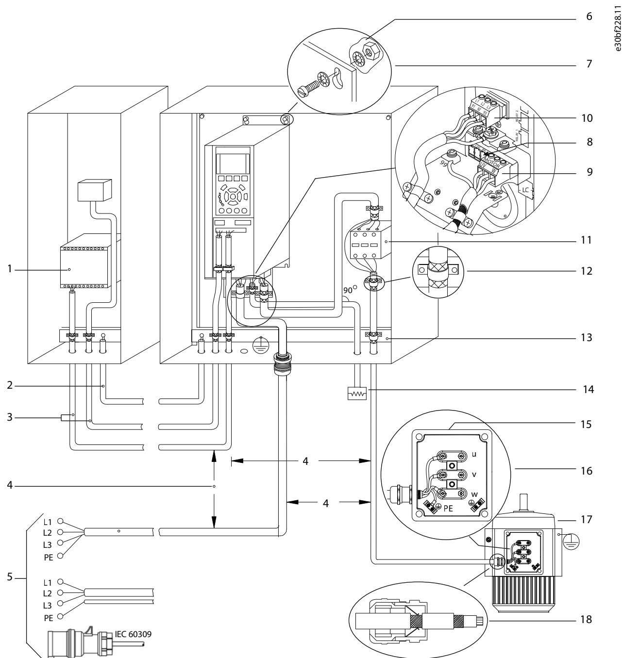
Illustration 60: EMC-compliant Electrical Connection
