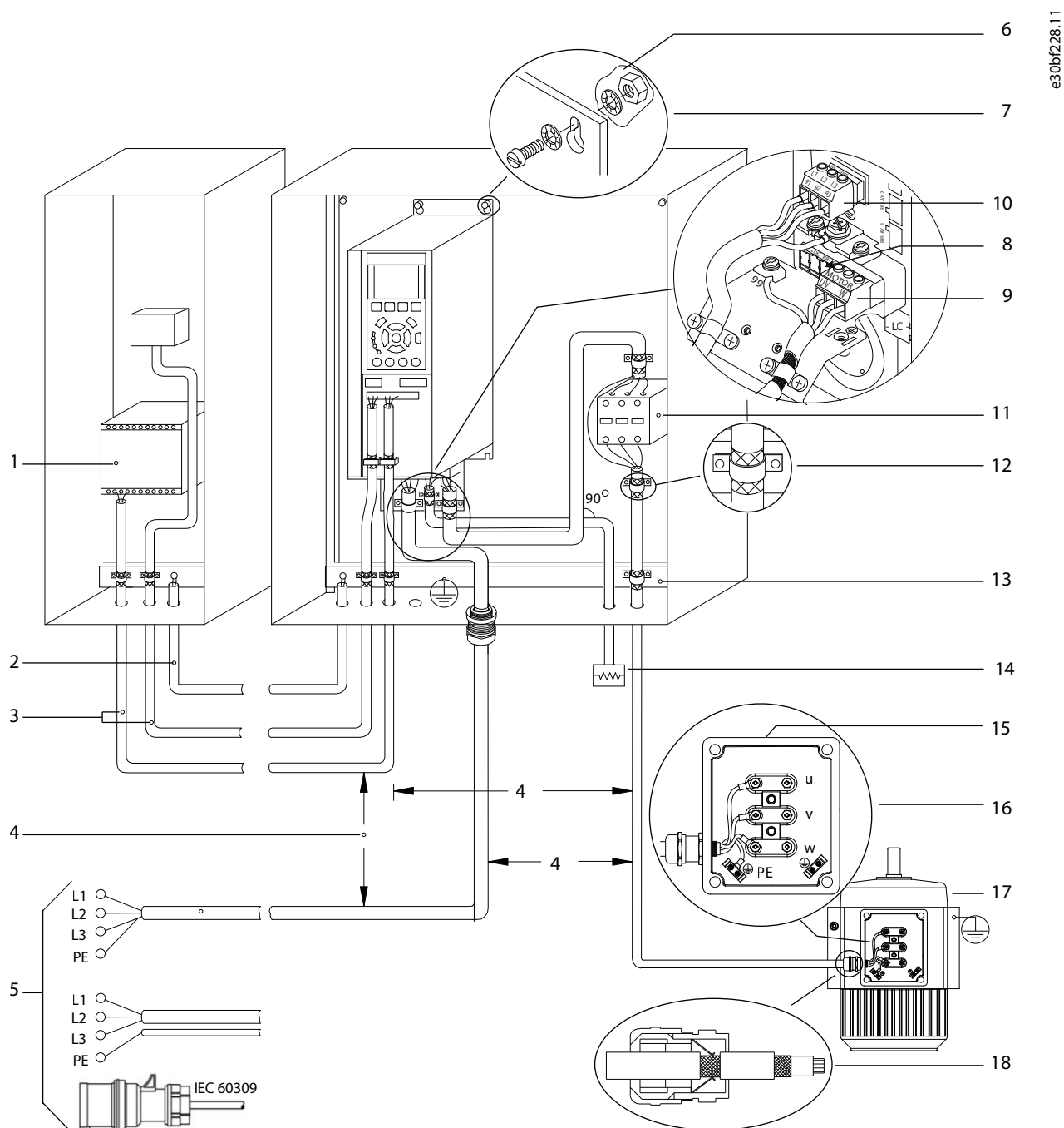
Illustration 81: Example of Proper EMC Installation
