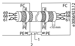
Illustration 66: Twisted-pair Cables
