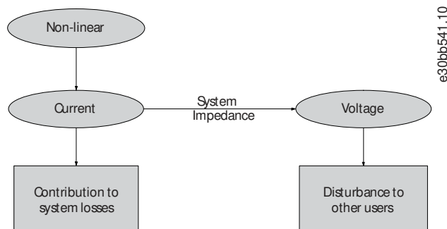
Illustration 83: Negative Effects of Harmonics
