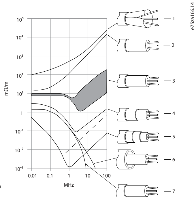
Illustration 63: Transfer Impedance ( Z_T )
