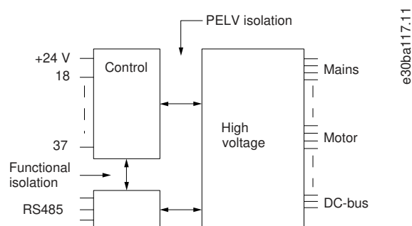
Illustration 53: PELV Isolation
