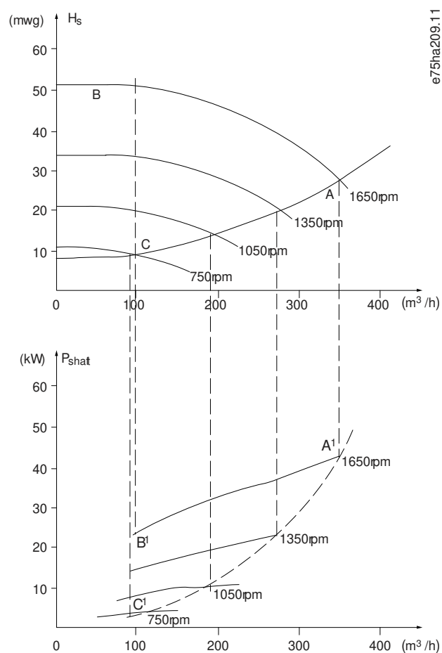
Illustration 12: Energy
