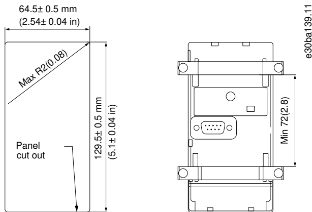
Illustration 51: Panel Mounting Kit Dimensions
