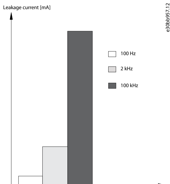
Illustration 78: Influence of Cut-off Frequency of the RCD on what is Responded to/Measured
