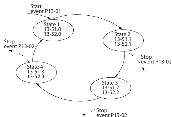
Illustration 34: Sequence with 4 Events/Actions
