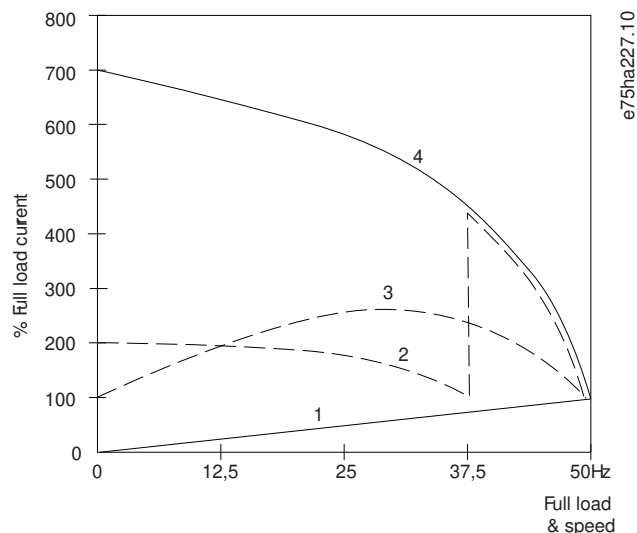
Illustration 13: Start-up Current
