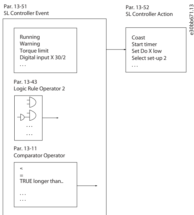
Illustration 33: Associated Action
