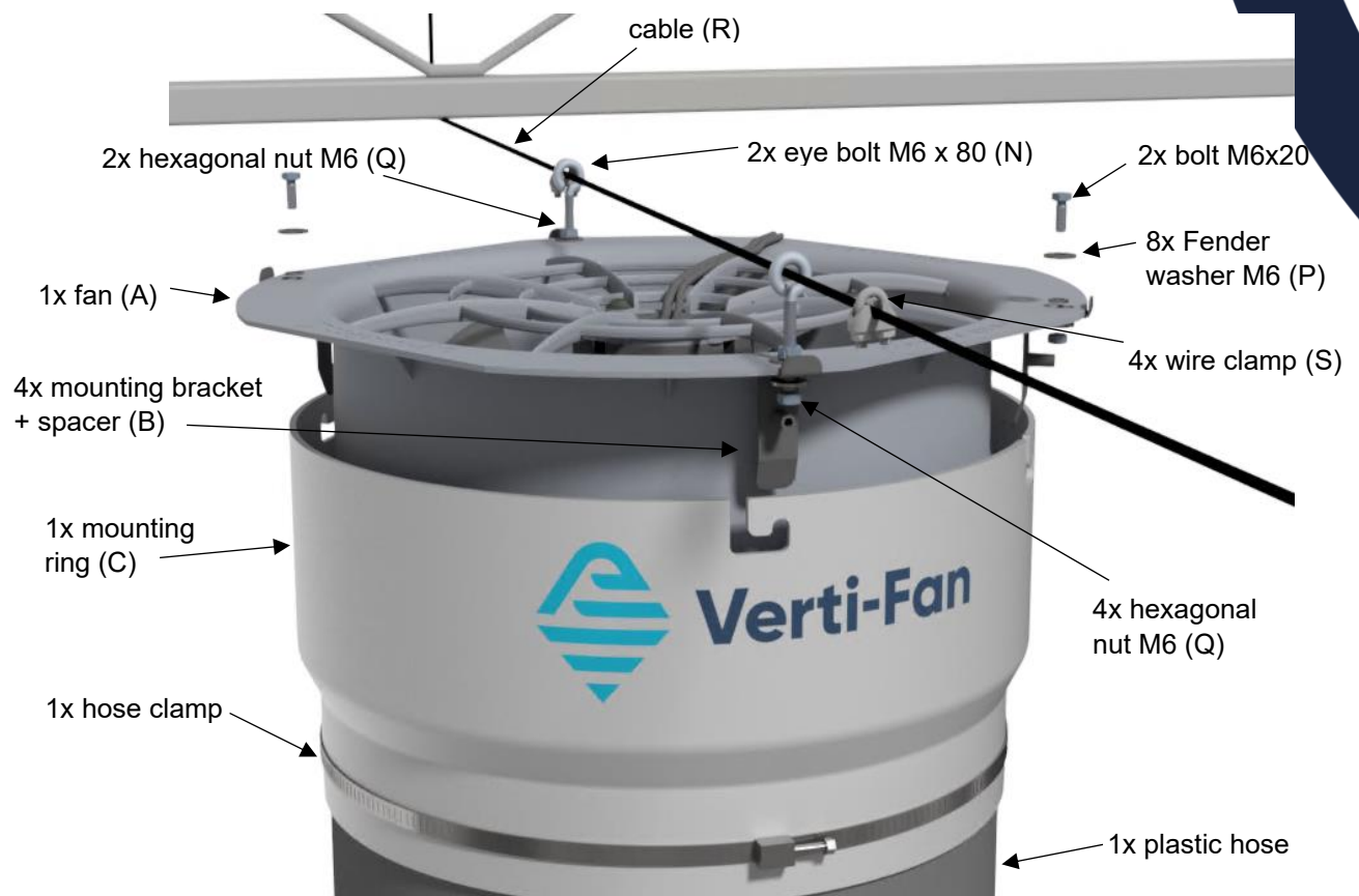
Figure 4 Verti-Fan suspended with aid of a steel cable
