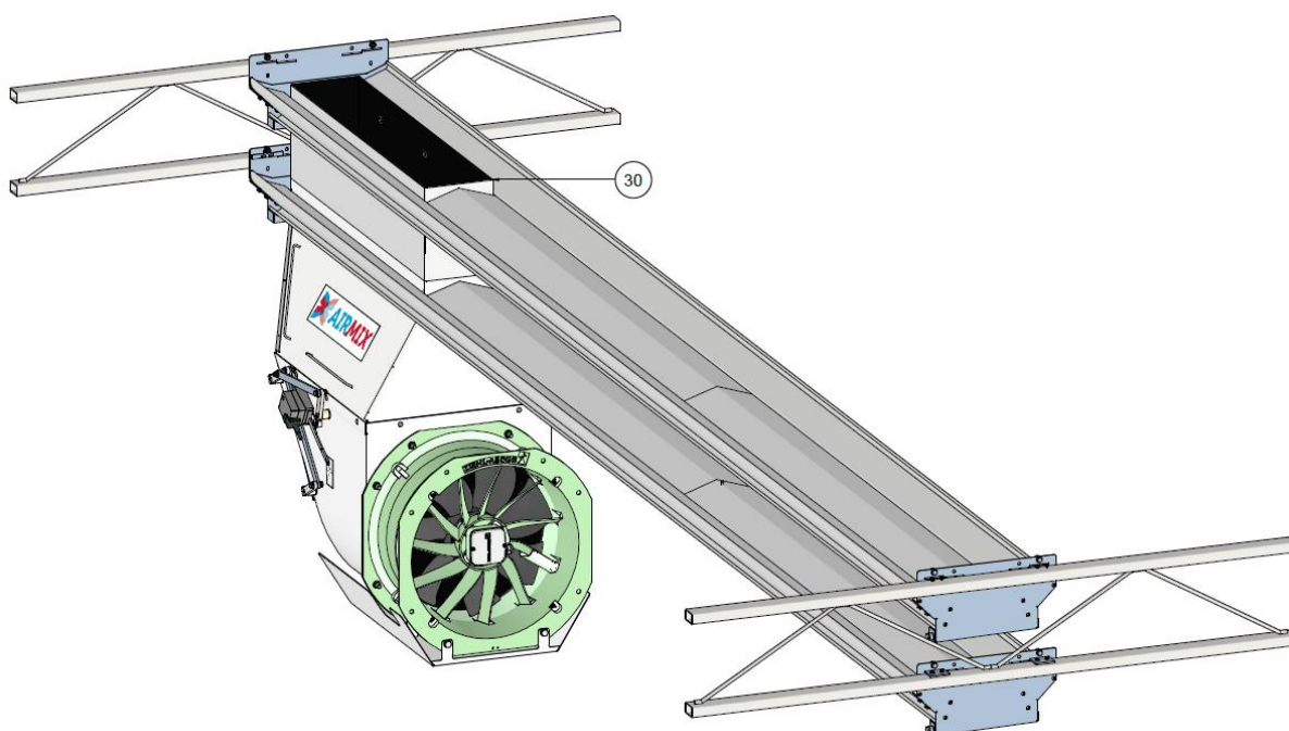
Figure 11 Installing the extension
