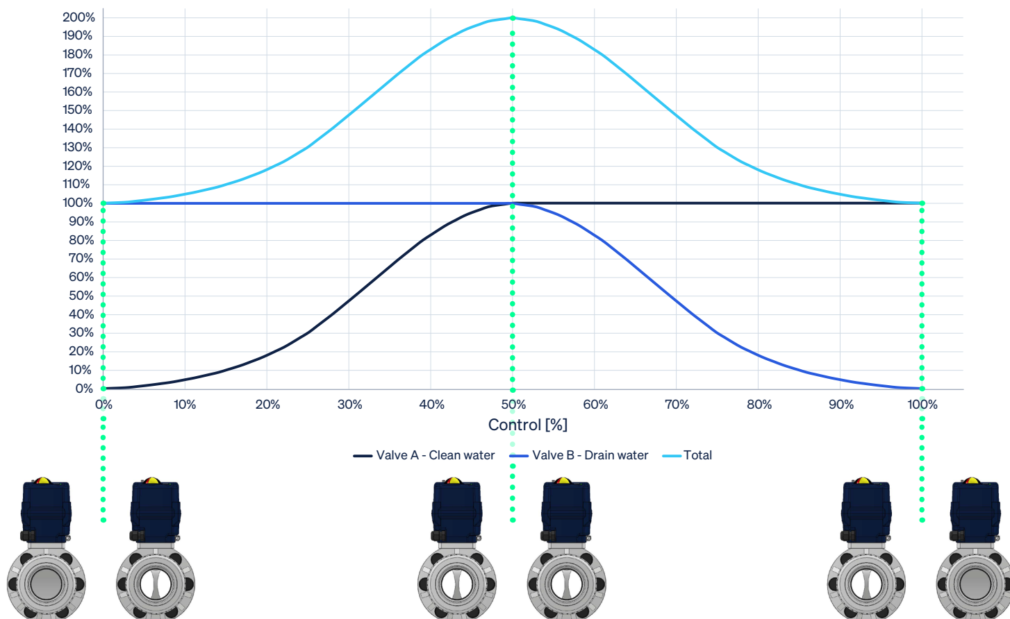
Flow characteristic of mixing valve - 200% control
