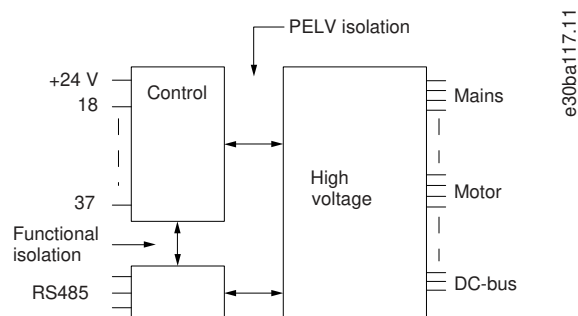
Illustration 53: PELV Isolation
