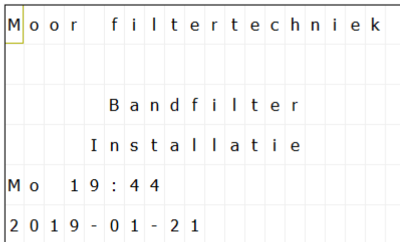
Figure 2: Start-up screen
