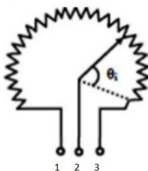
Figure 30 Schematic valve position sensor
