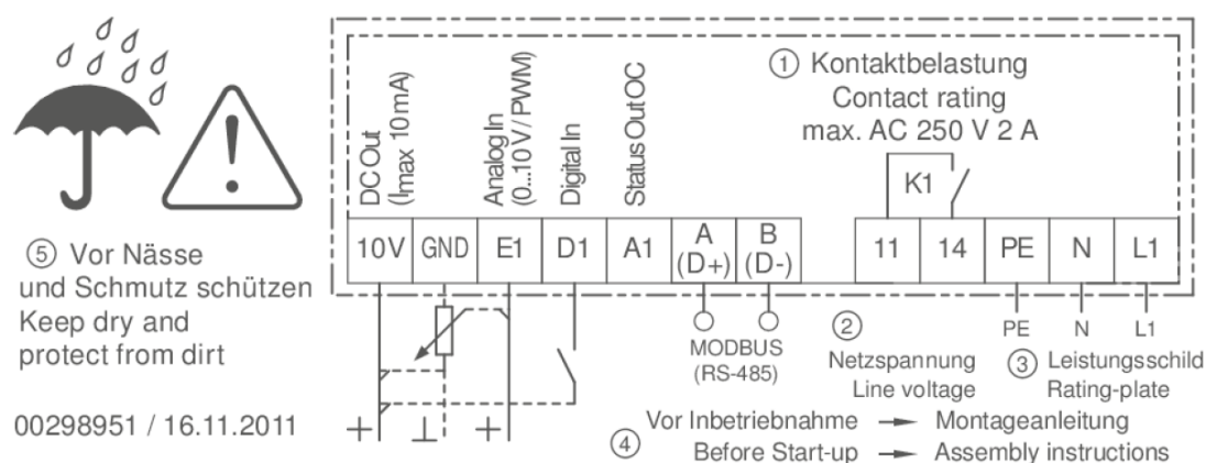
Figure 24 Connecting diagram ZN045-6IL
