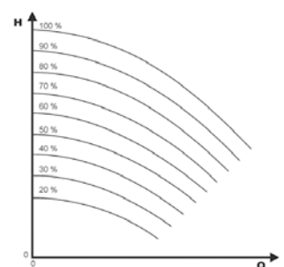
Control according to an external signal
