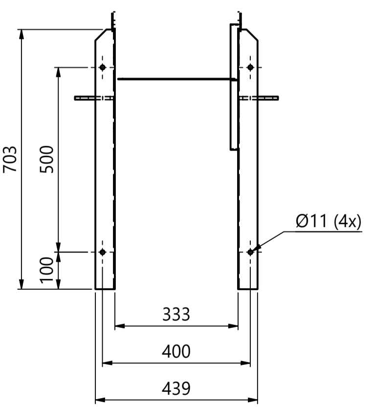
FUNDATIEPLAN FOUNDATION PLAN
