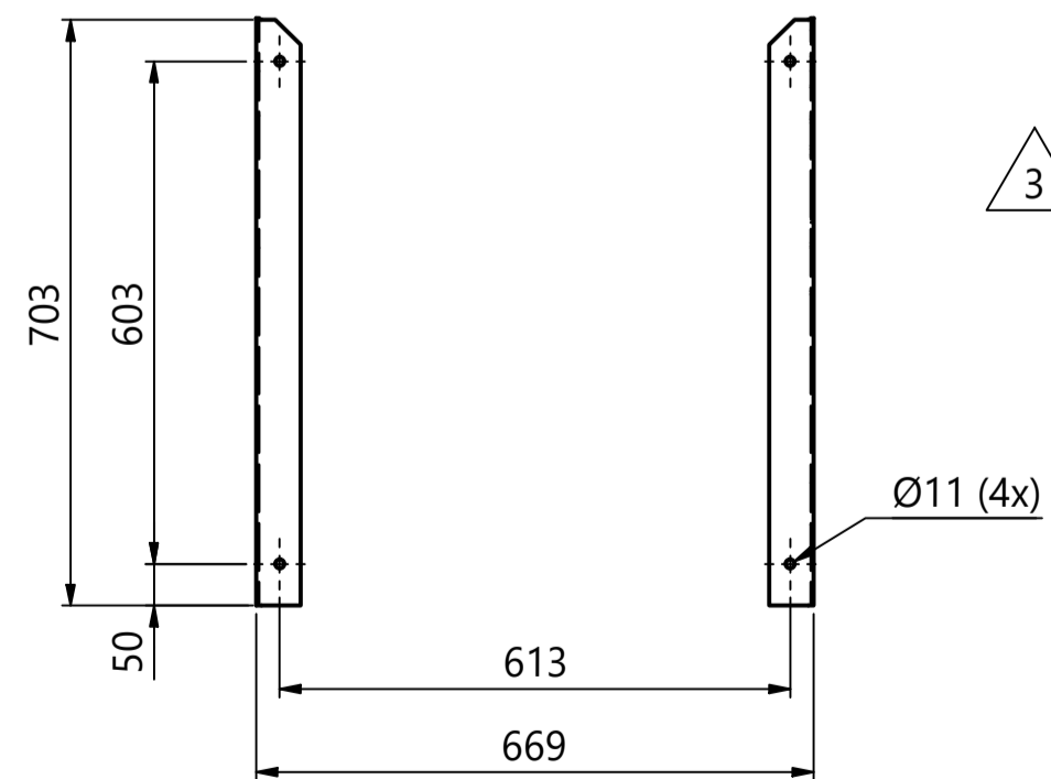
FUNDATIEPLAN FOUNDATION PLAN
