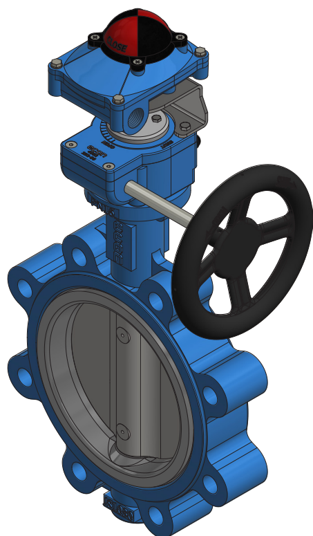
Fig. 6832 DN150 with gear box Fig. 4002 and switch box Fig. 79651
