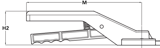
Aluminium lever - Fig. 4001K
